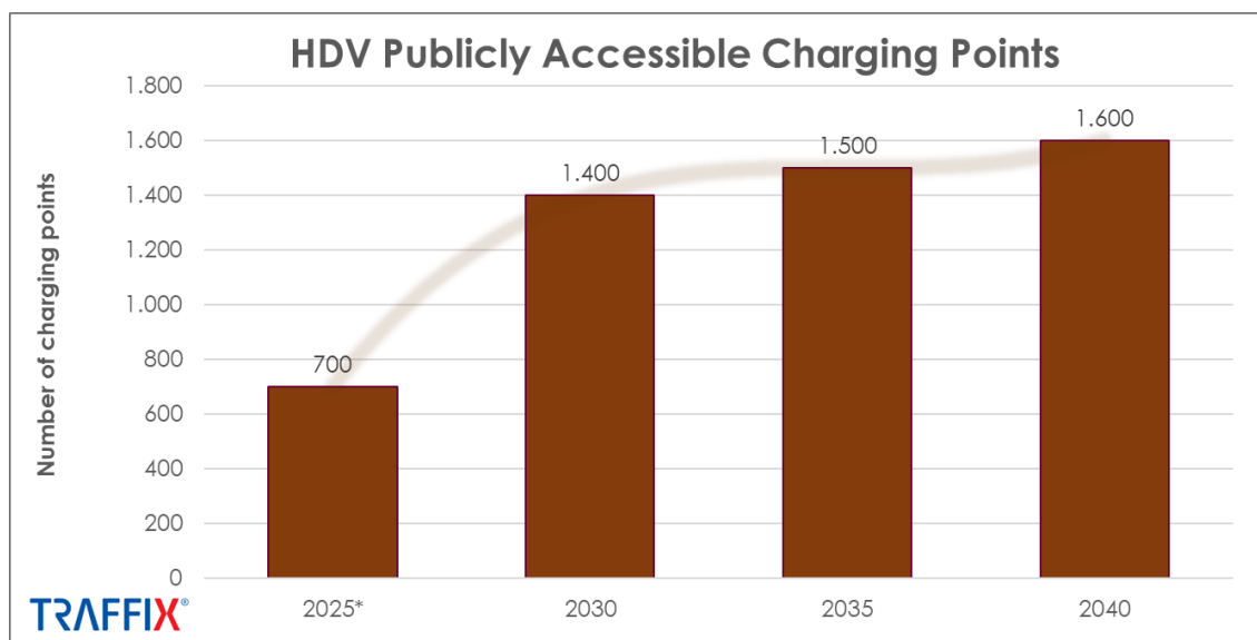
Figure 5-16: Projected demand for publicly accessible HDV charging points in Austria 2025-2040
