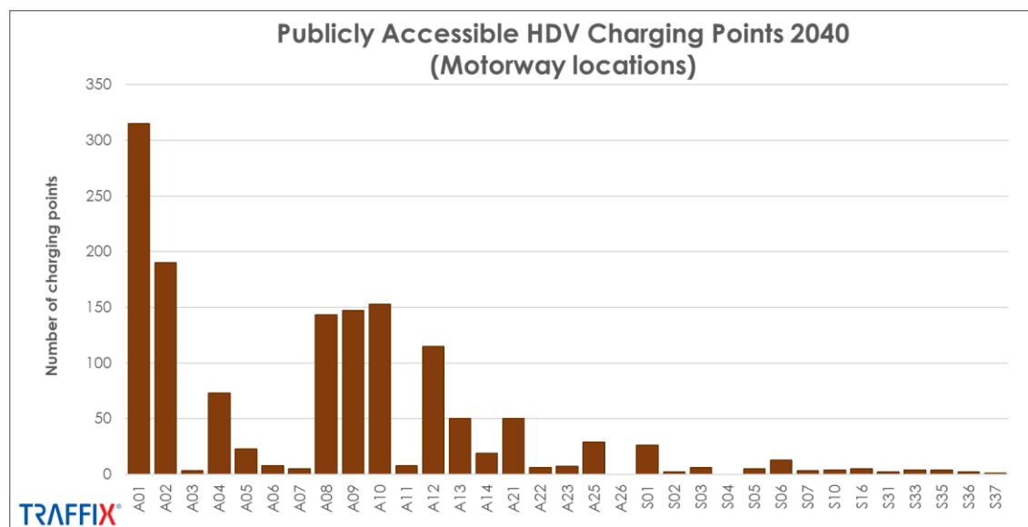
Figure 5-18: Demand for publicly accessible HDV range extension charging points 2040 by motorway
