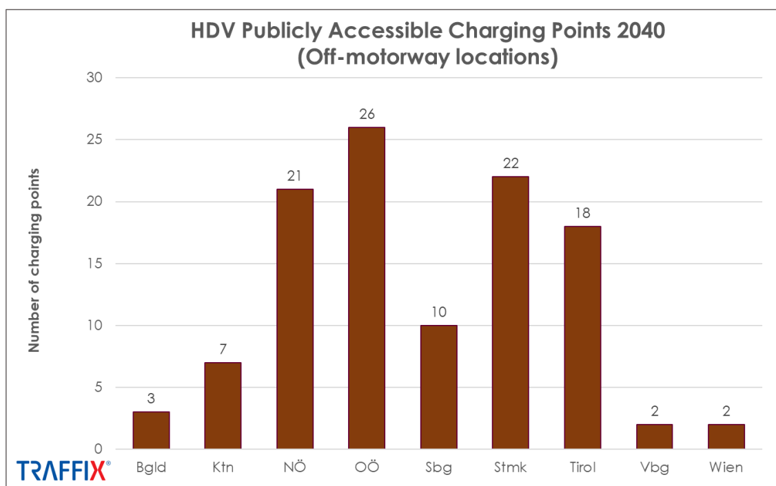
Figure 5-19: Demand for publicly accessible HDV range extension charging points 2040 by federal state (excluding locations on or near motorways)
